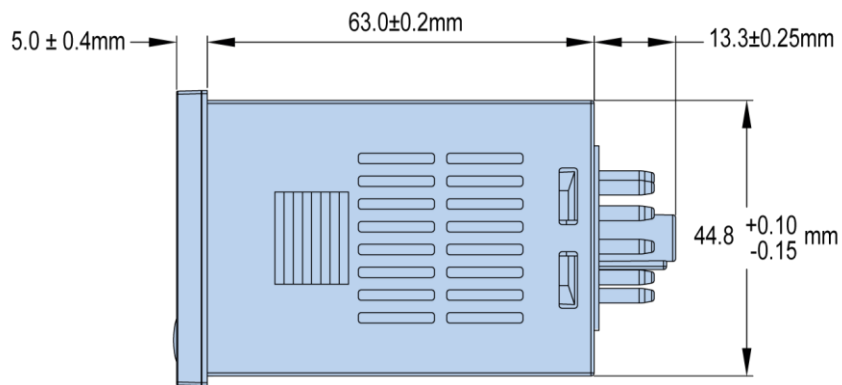
Mounting
