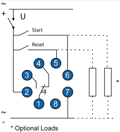
MDE1...MVA
