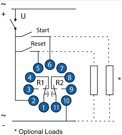
GDS2
