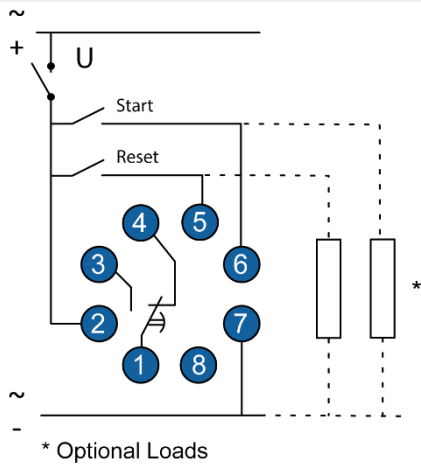
MDE1...24U
