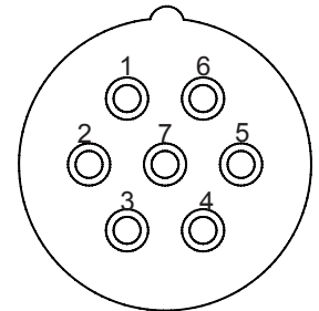
Femelle - Female - Buchse
