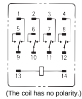
Terminal Arrangement/Internal Connections (Bottom View) Standard Models
