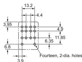
PCB Processing Dimensions (Bottom View)
