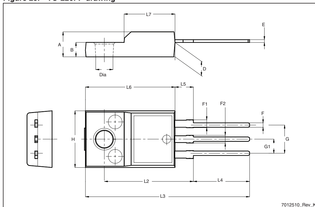
Figure 25. TO-220FP drawing
