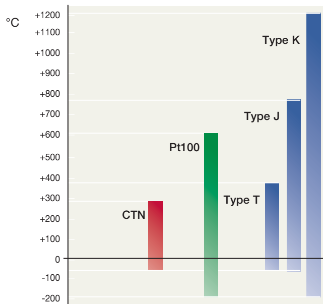
Legend: CTN (red), Pt100 (green), Thermocouple (blue)
