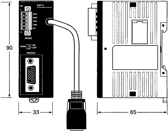
Interface RS-422/RS-232C (CPM2C-CIF11)
