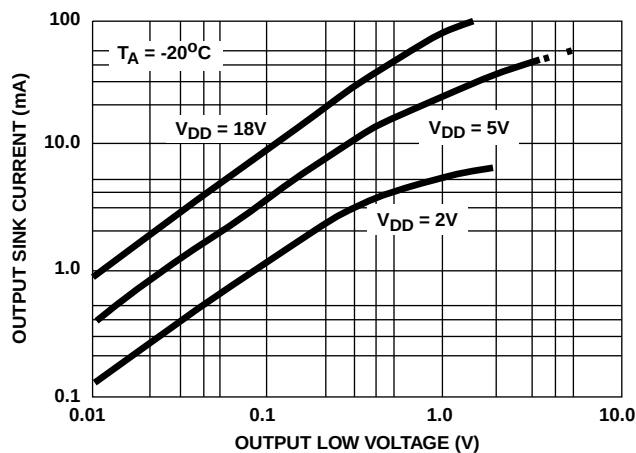
FIGURE 7. OUTPUT SINK CURRENT vs OUTPUT VOLTAGE
