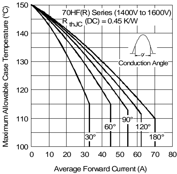
Fig. 3 - Current Ratings Characteristics
