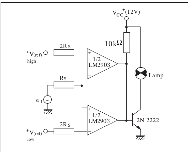
LIMIT COMPARATOR
