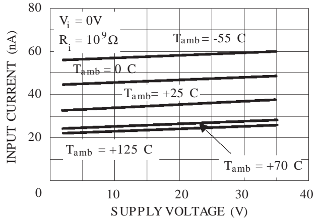
INPUT CURRENT versus SUPPLY VOLTAGE
