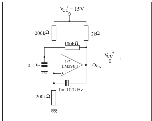
CRYSTAL CONTROLLED OSCILLATOR
