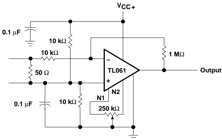
Figure 24. AC Amplifier
