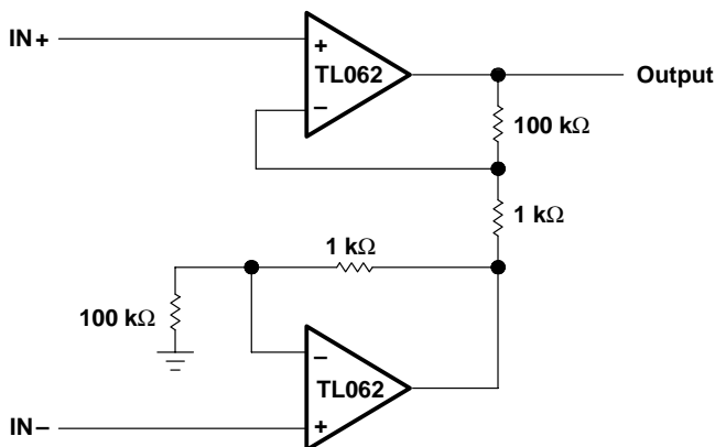
Figure 26. Instrumentation Amplifier
