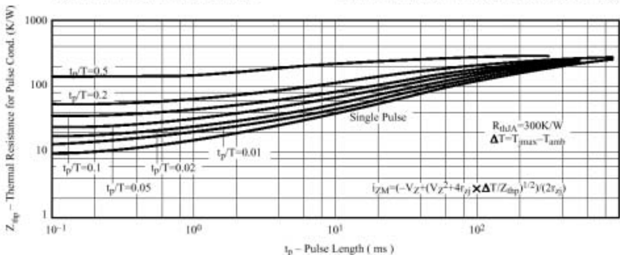
Figure 10. Thermal Response
